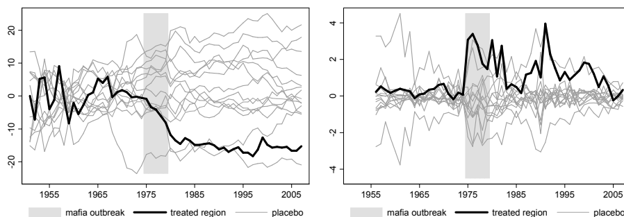
Figure 11: distribution of the estimated gap between each Italian region and its synthetic control in terms of GDP per capita and murders, years 1951-2007 (placebo test)
