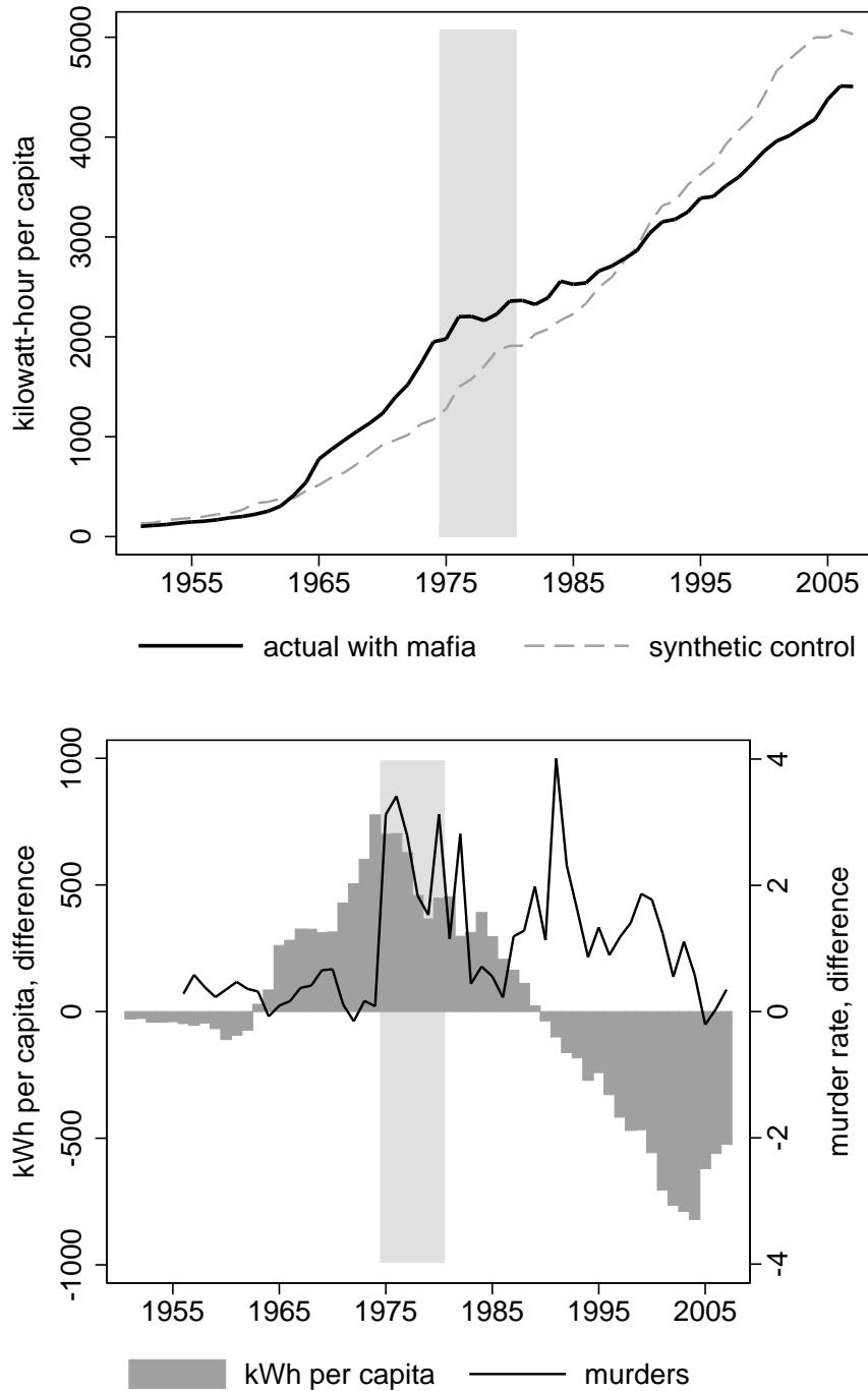
Figure 12: electricity consumption in the treated region and in the synthetic control, years 1951-2007
