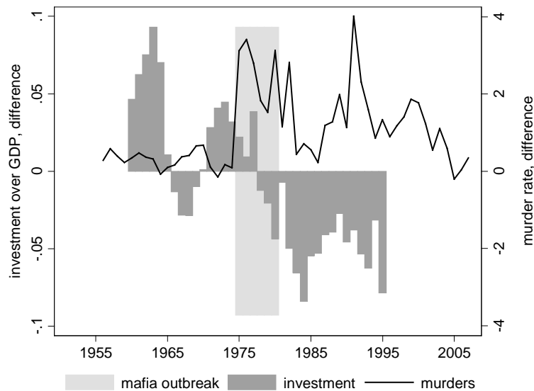
Figure 10: private investment and murder rate in the treated region and in the synthetic control, estimated gap, years 1956-2007
